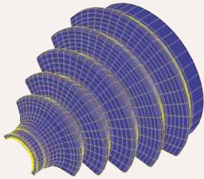
RUBBER BOOT HALF-MODEL
