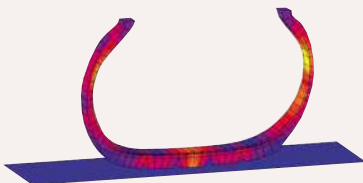
CONTACT OF TIRE SECTION
