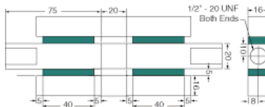
QUAD LAP SHEAR TEST
