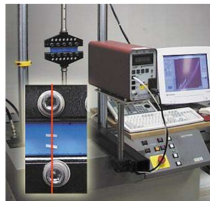
LASER EXTENSOMETER
