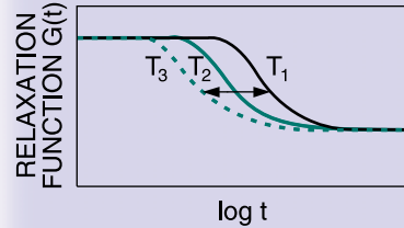
THERMO-RHEOLOGICALLY SIMPLE BEHAVIOR IN POLYMERS
