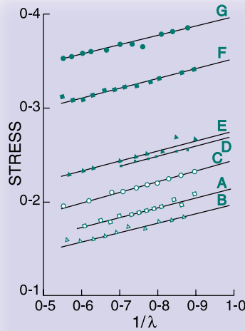
EXAMPLE 1: DETERMINATION OF MOONEY-RIVLIN CONSTANTS FOR VULCANIZED RUBBER IN SIMPLE TENSION
