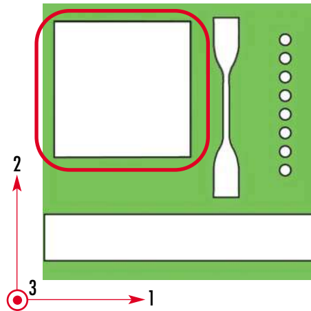
BIAXIAL SPECIMEN
