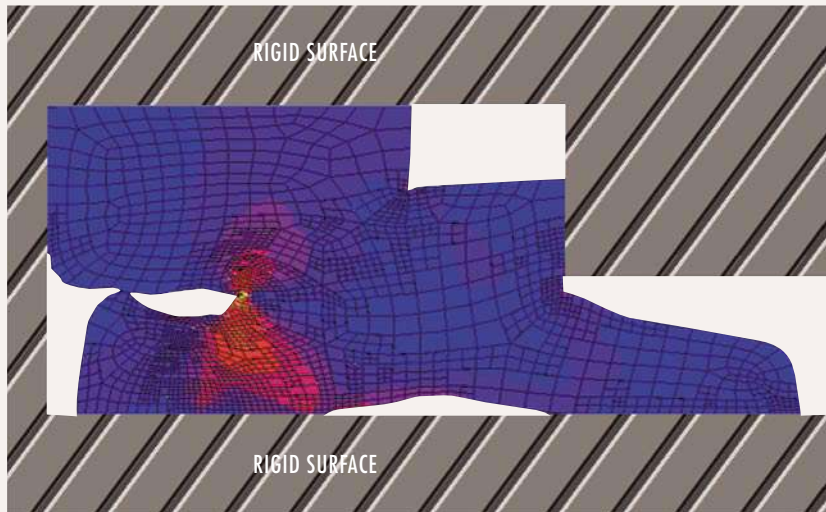
EQUIVALENT CAUCHY STRESSES: USING ADAPTIVE MESHING
