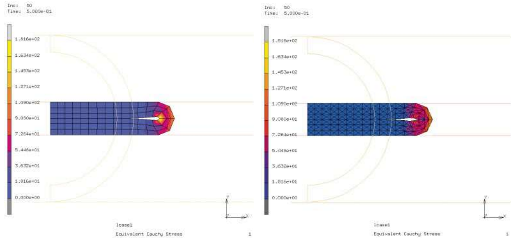
COMPRESSED TUBE USING QUADRILATERALS AND TRIANGLES
