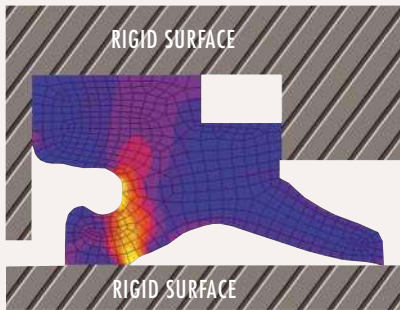
EQUIVALENT CAUCHY STRESSES: INCREMENT 20
