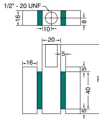
DUAL LAP SHEAR TEST
