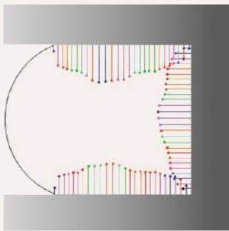
CONTACT FORCES DISTRIBUTION (INCREMENT 70)
