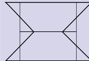
2-D HOURGLASSING MODE
