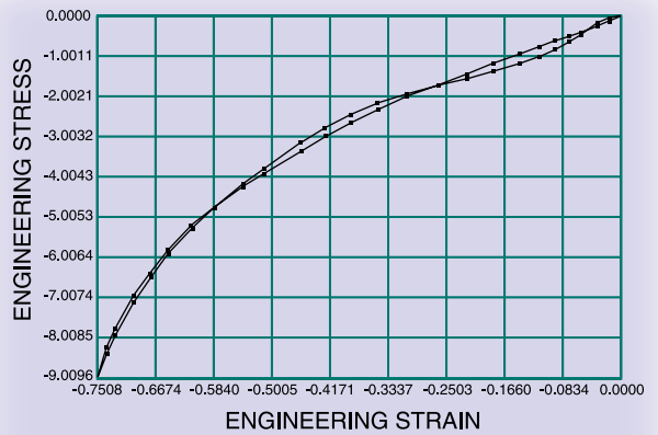
EXAMPLE 3: CURVE FIT TO FOAM DATA
