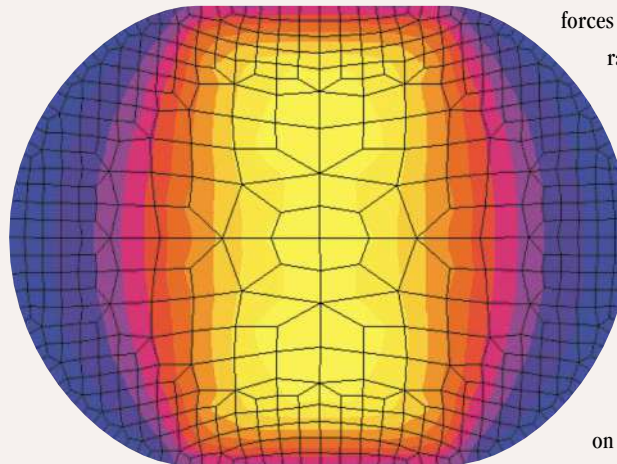
CAUCHY STRESSES IN RADIAL DIRECTION (INCREMENT 20)
