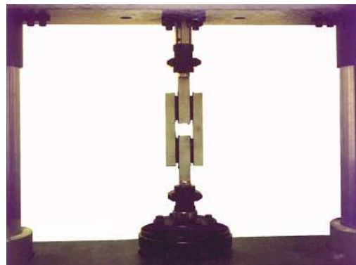
DUAL LAP SHEAR TEST
