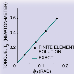
FINITE ELEMENT SOLUTION: TORQUE VS. TWIST. From Morman and Nagtegaal [1983].
