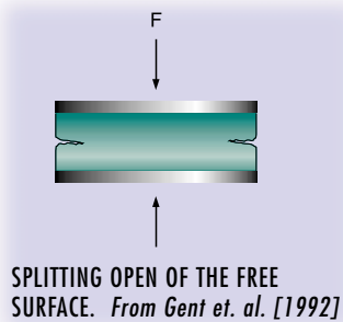
TWO POSSIBLE FRACTURE MODES UNDER STATIC COMPRESSION
