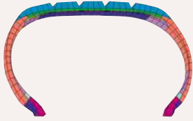
TIRE SECTION SHOWING DIFFERENT MATERIALS
