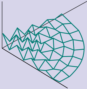
3-D HOURGLASSING: "EGGCRATE" MODE
