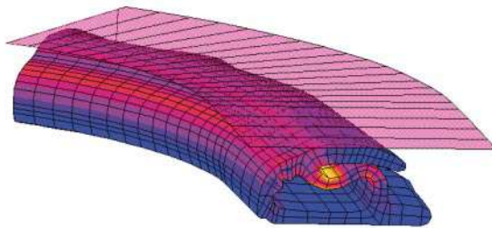
RUBBER SEAL SUBJECTED TO CONTACT SURFACES
