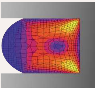
FINAL DEFORMED GEOMETRY (INCREMENT 70)
