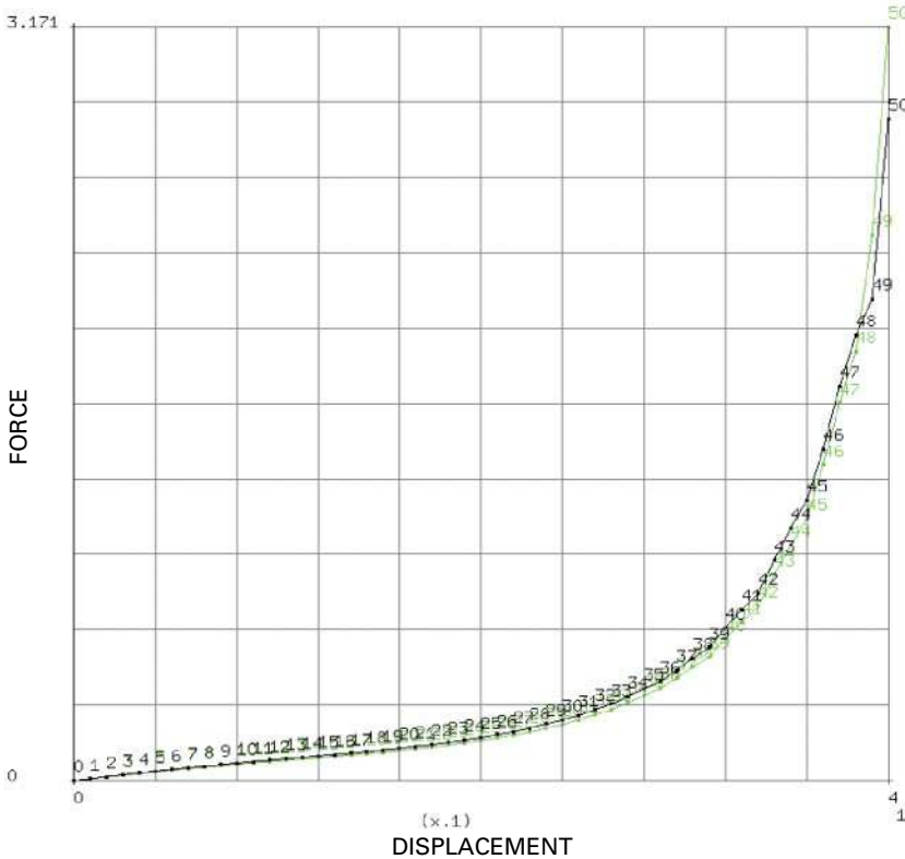
GENERALIZED XY PLOT TO COMPARE QUAD AND TRI RESULTS
