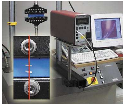
LASER EXTENSOMETER WITH TAGS ON SPECIMEN
