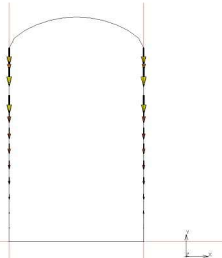
CONTACT FRICTION FORCE
