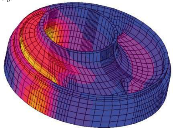
RUBBER BUSHING
