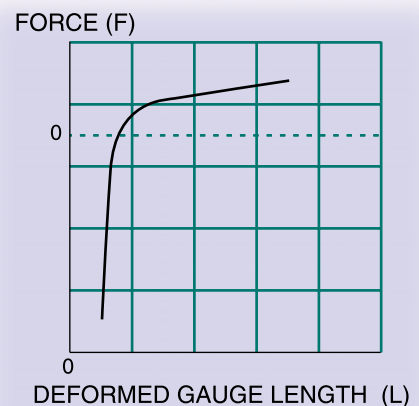
BLATZ-KO MODEL FOR FOAMS
