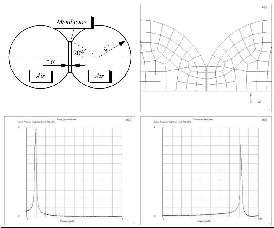
Coupled Structural - Acoustic Analysis
