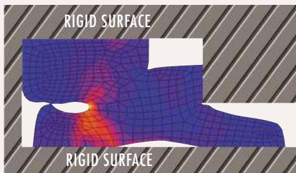
EQUIVALENT CAUCHY STRESSES: INCREMENT 40
