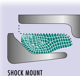
SHOCK MOUNT
