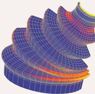
AXIAL COMPRESSION (INCREMENT 13)
