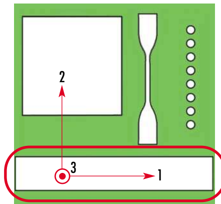
PLANAR SHEAR SPECIMEN
