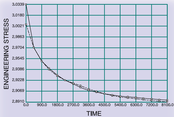
EXAMPLE 4:: CURVE FIT TO VISCOELASTIC RELAXATION DATA
