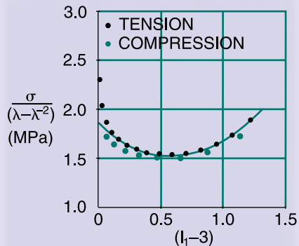
YEOH MODEL: TENSILE AND COMPRESSIVE DATA REPLOTTED AGAINST (I_1 - 3) . From Yeoh [1990].
