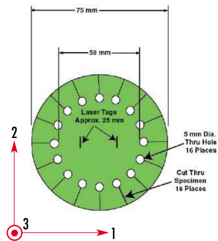
BIAXIAL SPECIMEN
