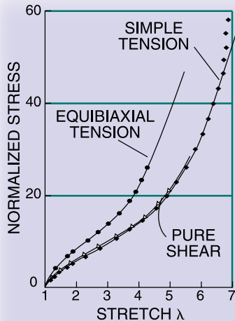
EXAMPLE 2: CORRELATION OF 3-TERM OGDEN MODEL WITH TRELOAR'S DATA IN SIMPLE TENSION, PURE SHEAR, AND EQUIBIAXIAL TENSION. From Ogden [1972].
