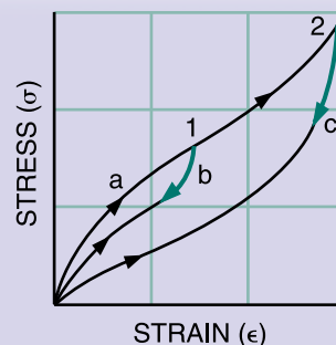
CYCLIC TENSION TEST DEMONSTRATING MULLINS' EFFECT. From Govindjee and Simo [1992].
