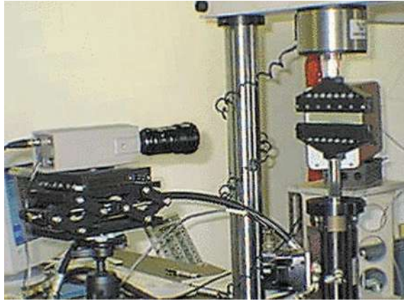
VIDEO EXTENSOMETER
